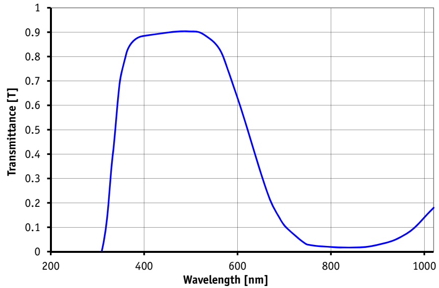
Figure 51: Approximate spectral transmission of IR cut filter type Hoya C-5000 (may vary slightly by filter lot)
