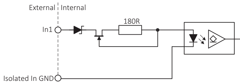
Figure 54: Input block diagram
