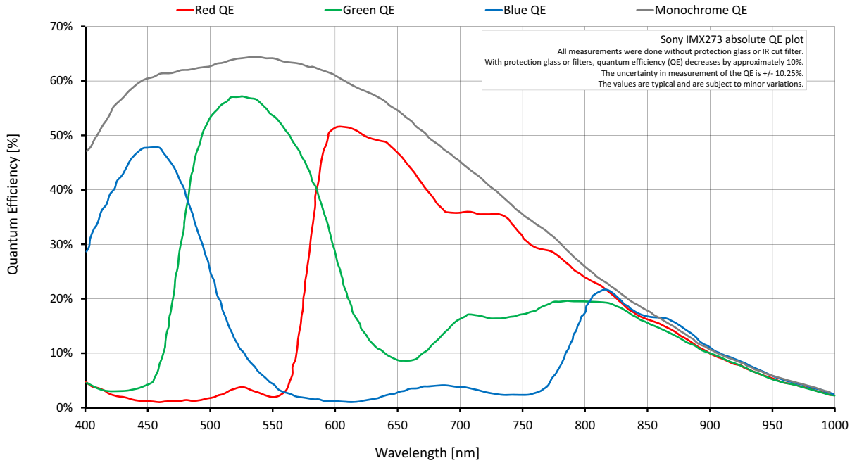
Figure 15: Mako G-158 (Sony IMX273) absolute QE
