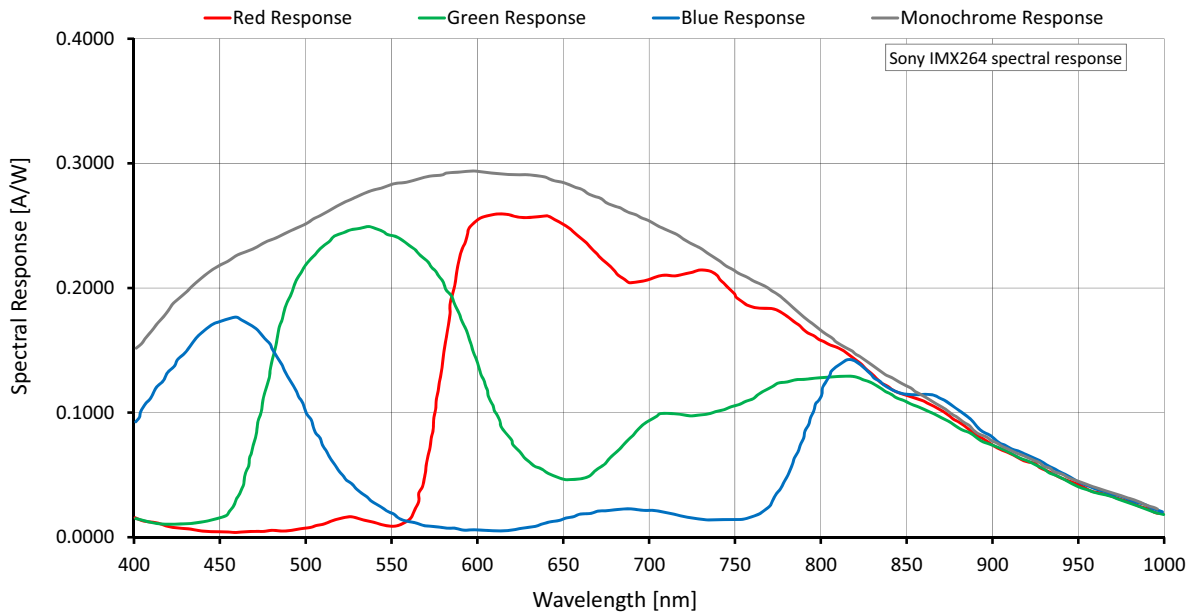
Figure 36: Mako G-507 (Sony IMX264) spectral response
