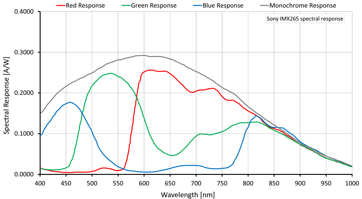
Figure 28: Mako G-319 (Sony IMX265) spectral response
