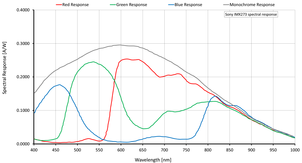
Figure 16: Mako G-158 (Sony IMX273) spectral response
