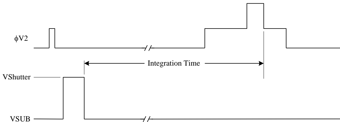
Figure 34: Integration Time Definition
