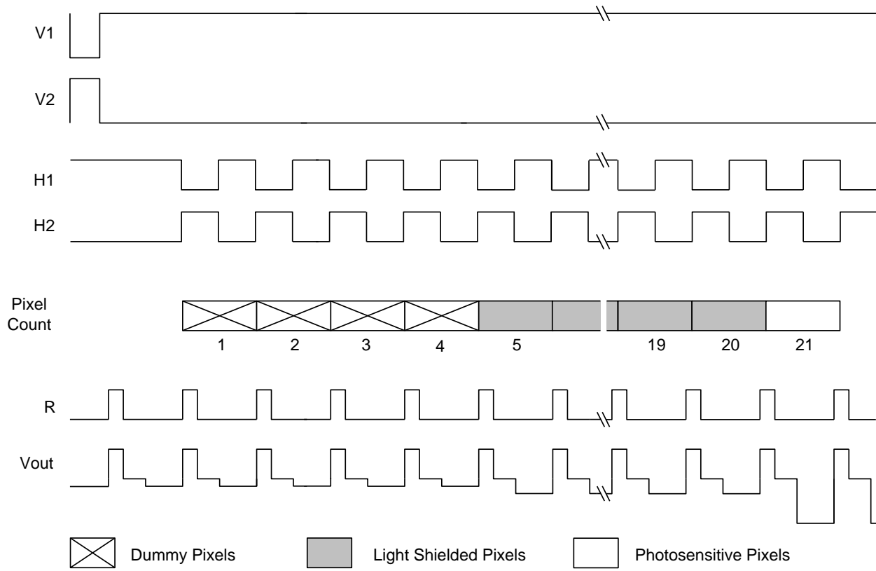
Figure 30: Pixel Timing
