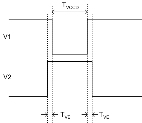
Figure 29: Line Timing Edge Alignment
