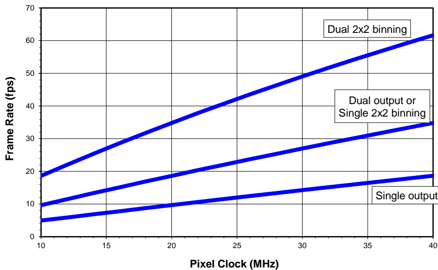
Figure 15: Frame Rates
