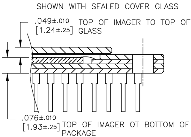
Figure 36: Completed Assembly (2 of 2)
