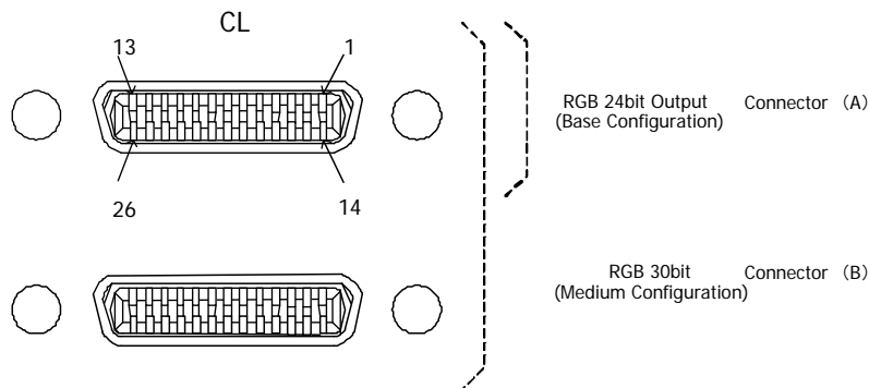
Connector (B)
