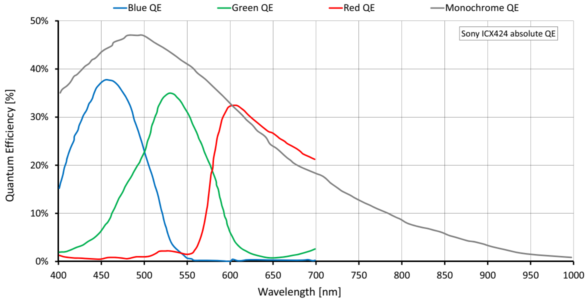
Figure 6: Mako G-032 (Sony ICX424) absolute QE
