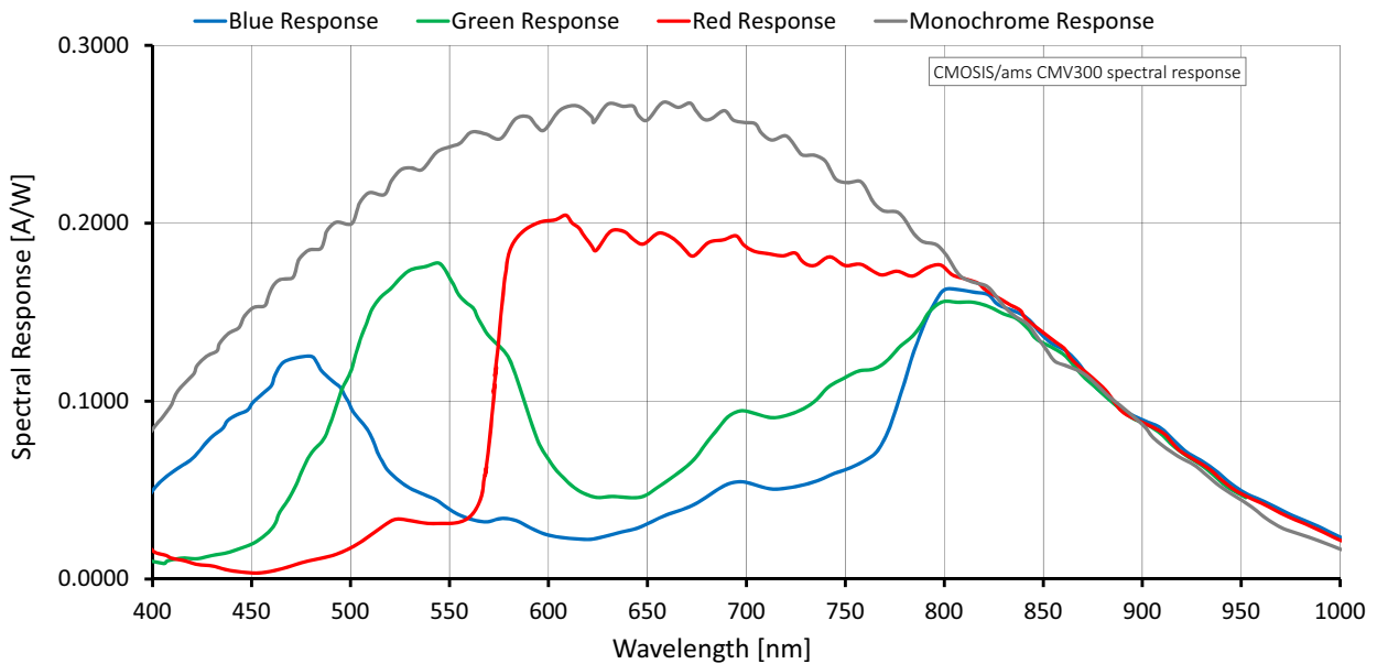
Figure 4: Mako G-030 (CMOSIS/ams CMV300) spectral response
