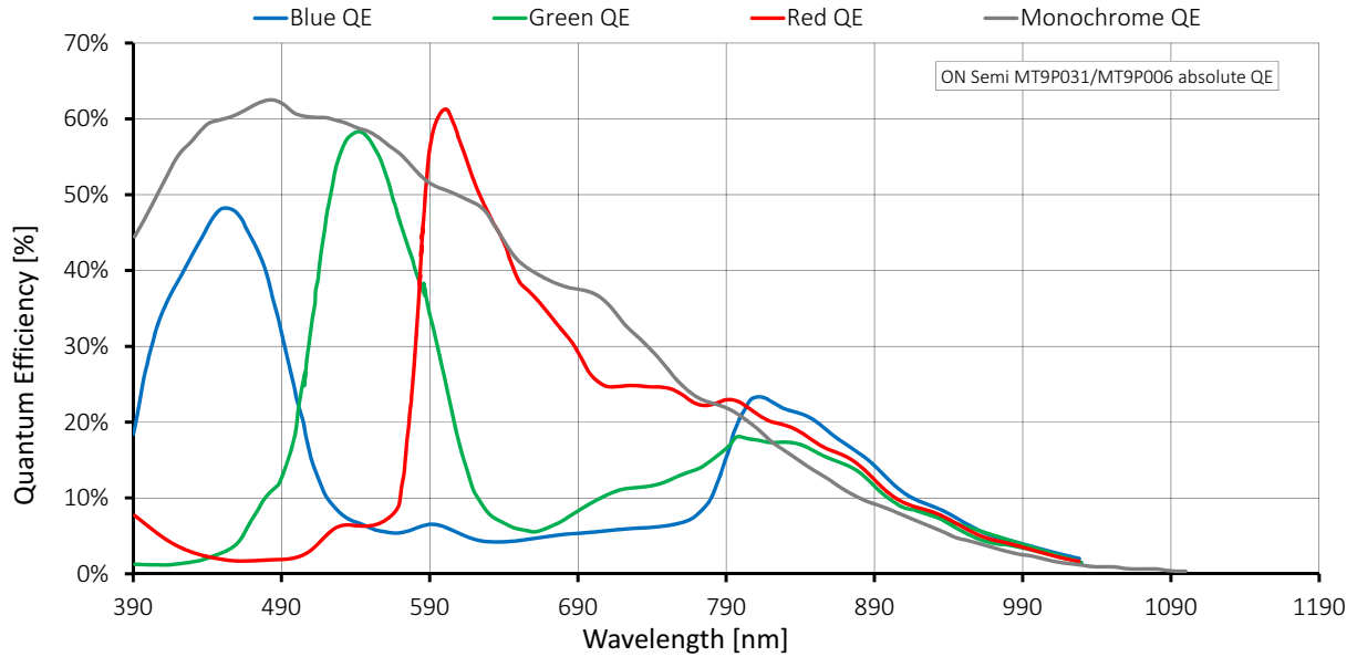
Figure 41: Mako G-503 (ON Semi MT9P031/MT9P006) absolute QE
