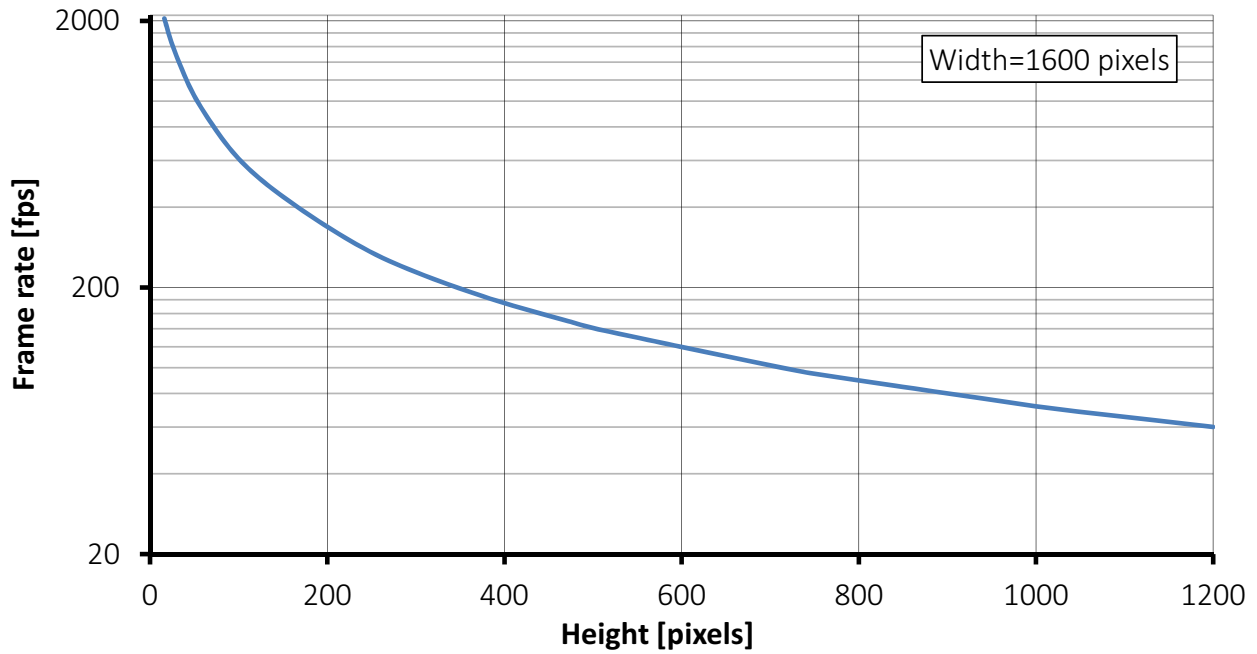
Figure 23: Mako G-192 frame rate as a function of ROI height
