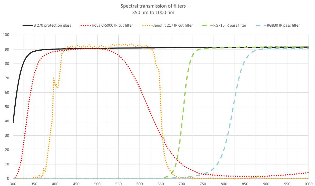
Figure 61: Optical filter spectral transmission
