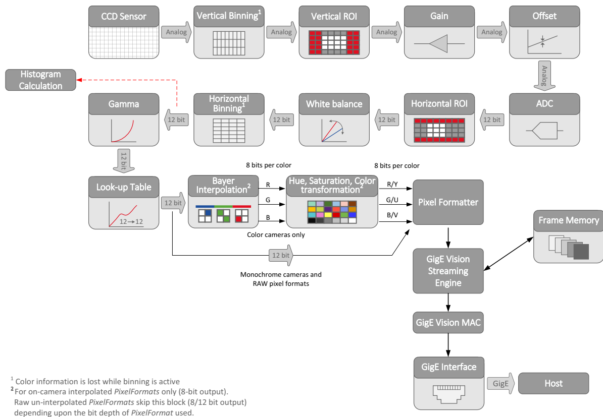
Figure 72: Mako G-032 and G-125 series image data flow
