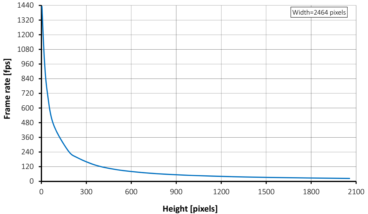
Figure 50: Mako G-508B POL frame rate as a function of ROI height
