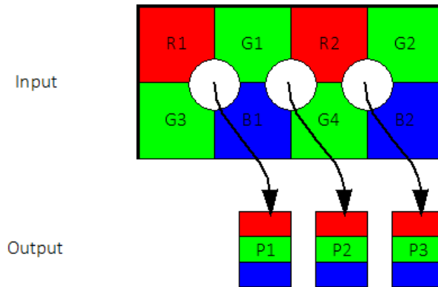
Figure 79: Bayer demosaicing (interpolation)
