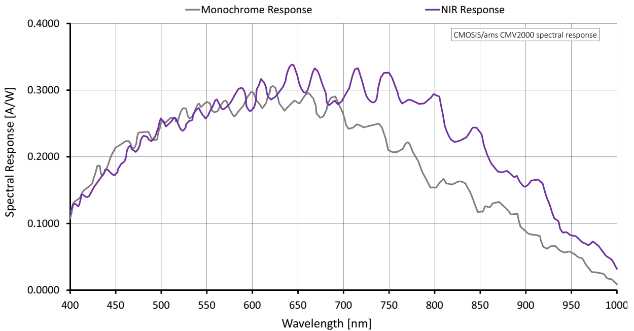
Figure 27: Mako G-223B NIR (CMOSIS/ams CMV2000) spectral response
