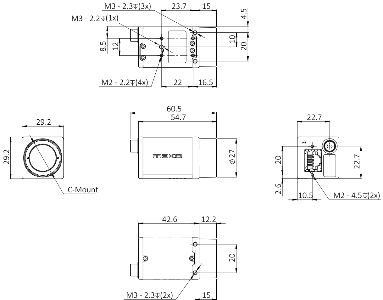
Figure 51: Mako G with C-Mount dimensions (including connectors)
