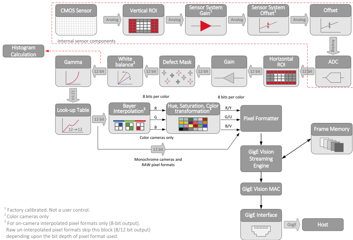
Figure 75: Mako G-223 and G-419 series image data flow
