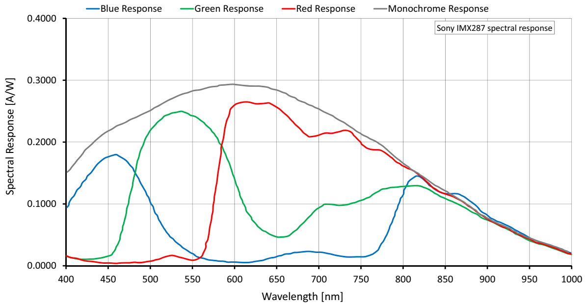
Figure 10: Mako G-040 (Sony IMX287) spectral response
