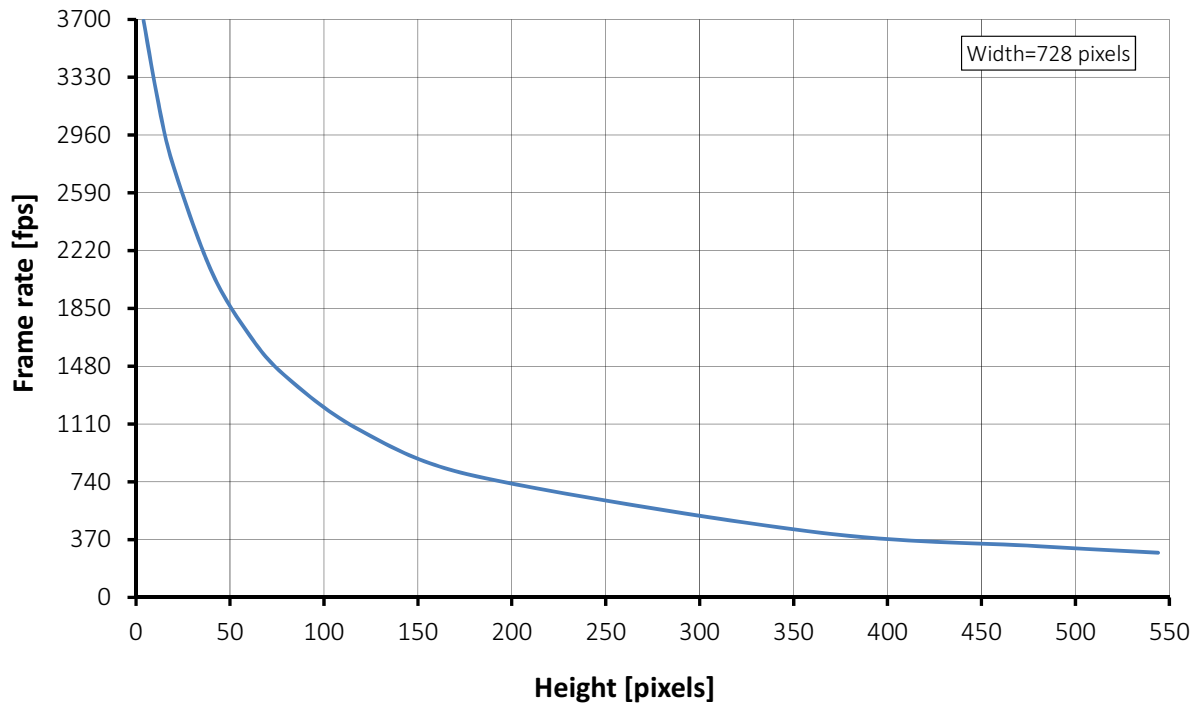
Figure 11: Mako G-040 frame rate as a function of ROI height
