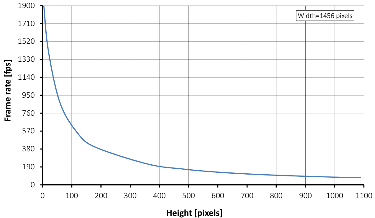
Figure 20: Mako G-158 frame rate as a function of ROI height
