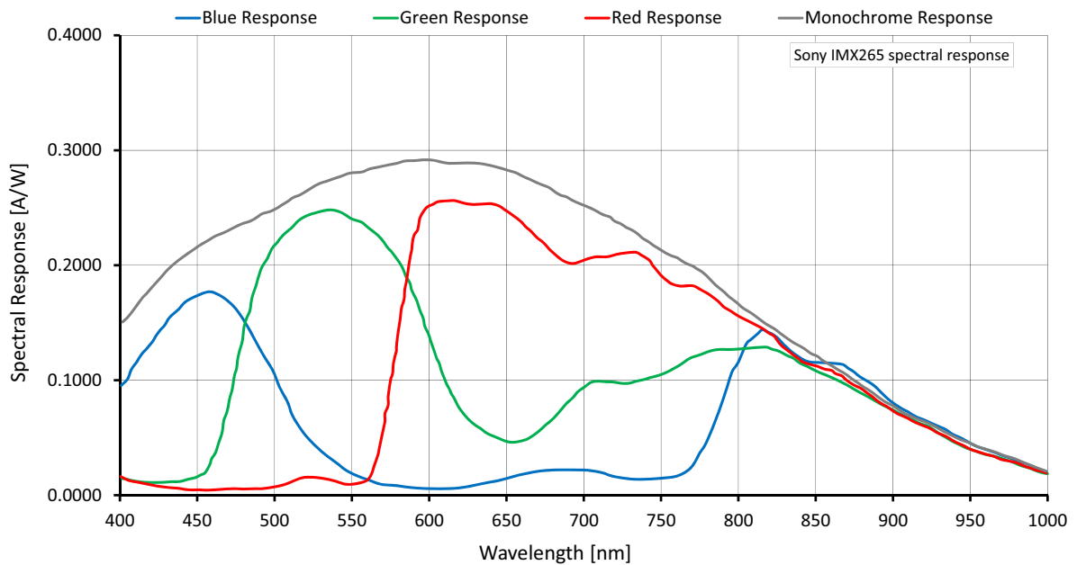
Figure 34: Mako G-319 (Sony IMX265) spectral response
