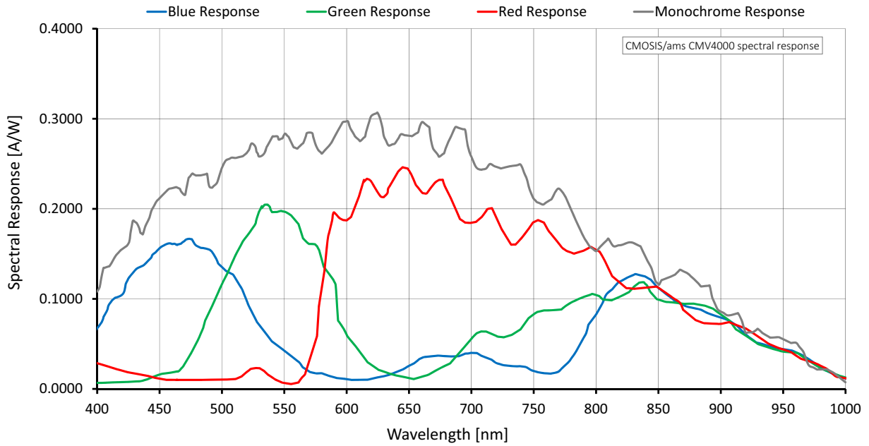
Figure 38: Mako G-419 (CMOSIS/ams CMV4000) spectral response
