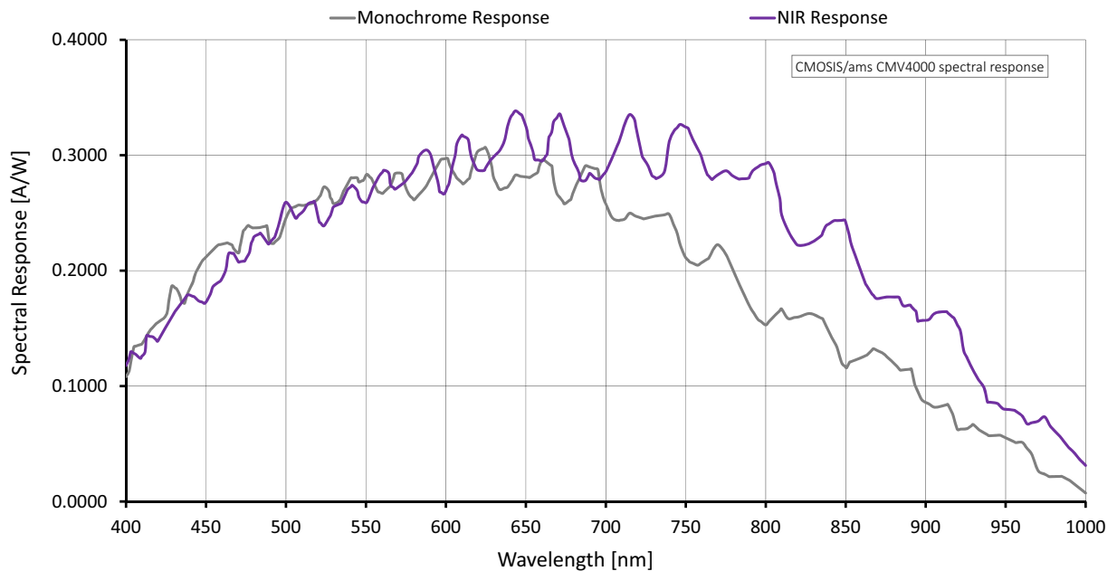
Figure 39: Mako G-419B NIR (CMOSIS/ams CMV4000) spectral response
