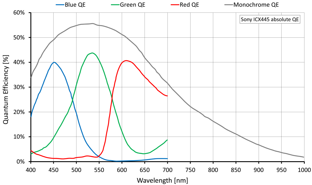
Figure 12: Mako G-125 (Sony ICX445) absolute QE
