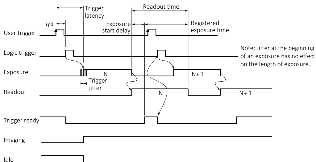
Figure 71: Internal signal timing waveforms (CMOS-sensor models)
