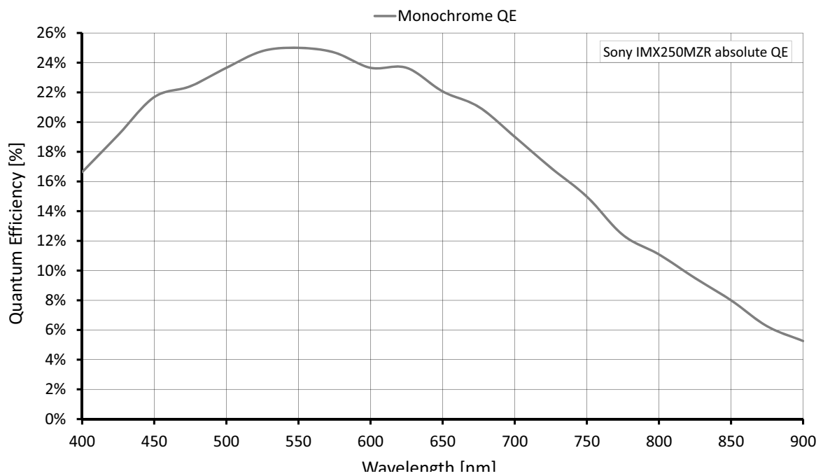
Figure 48: Mako G-508B POL (Sony IMX250MZR) spectral response
