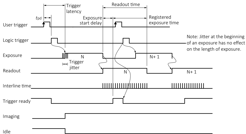
Figure 70: Internal signal timing waveforms (CCD-sensor models)
