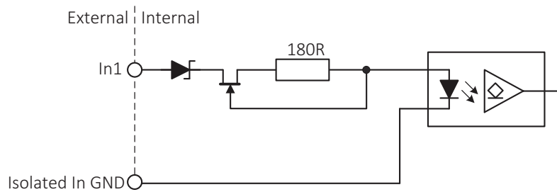
Figure 64: Input block diagram
