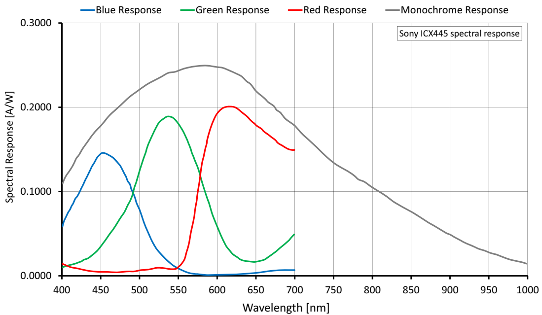
Figure 13: Mako G-125 (Sony ICX445) spectral response
