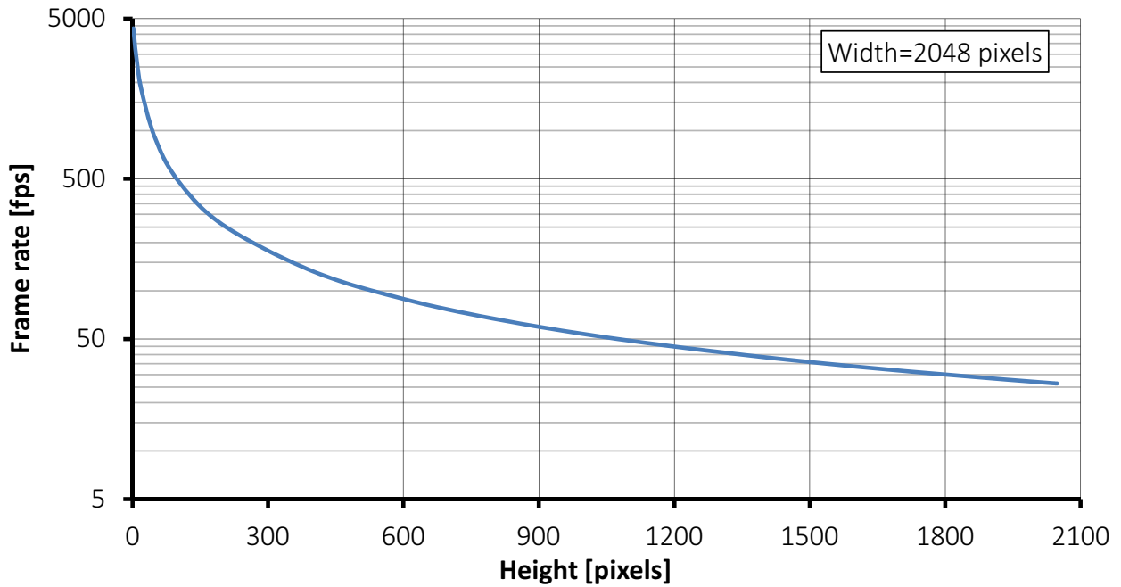
Figure 40: Mako G-419 frame rate as a function of ROI height
