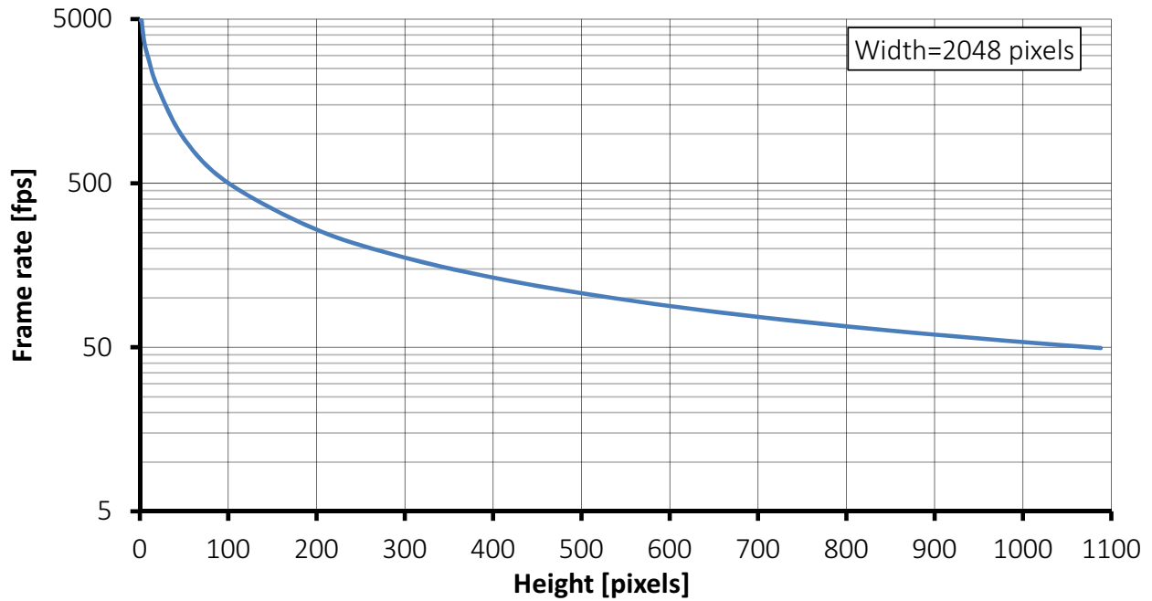
Figure 28: Mako G-223 frame rate as a function of ROI height
