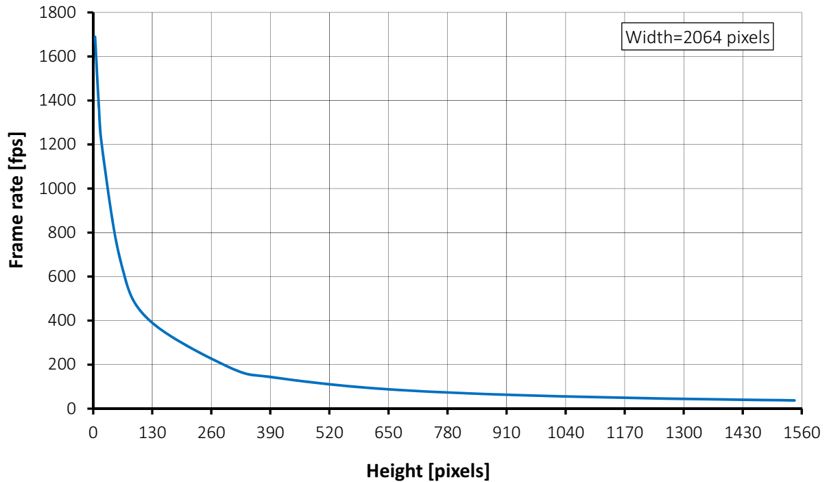
Figure 35: Mako G-319 frame rate as a function of ROI height
