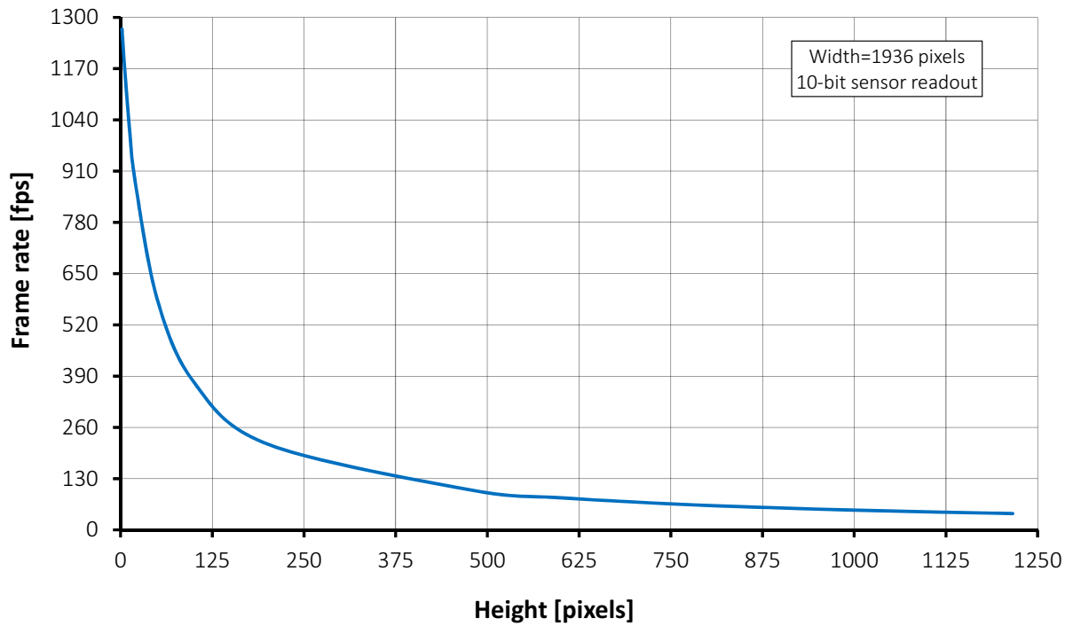
Figure 32: Mako G-234 10-bit sensor frame rate as a function of ROI height
