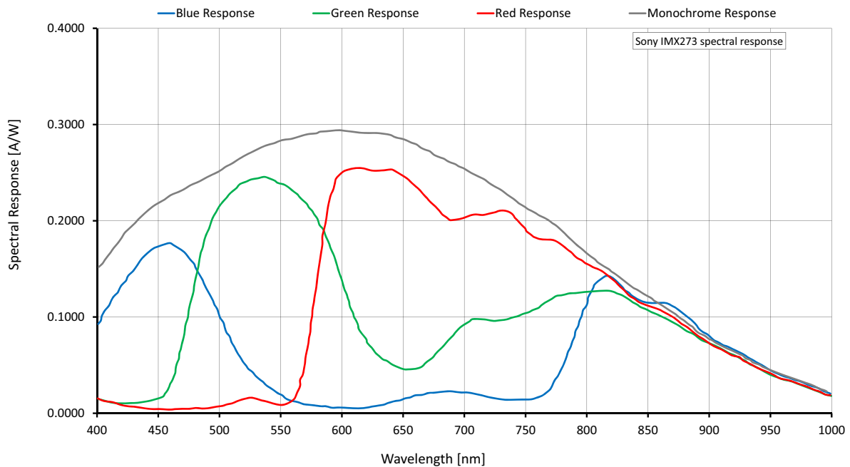
Figure 19: Mako G-158 (Sony IMX273) spectral response
