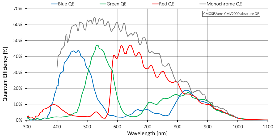
Figure 24: Mako G-223 (CMOSIS/ams CMV2000) absolute QE
