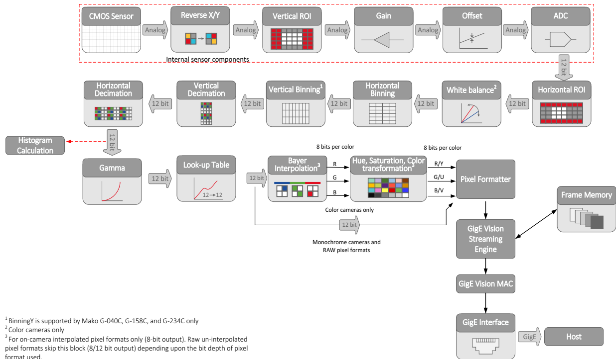
Figure 76: Mako G-040, G-158, G-234, G-319, G-507 series and G-508B POL image data flow
