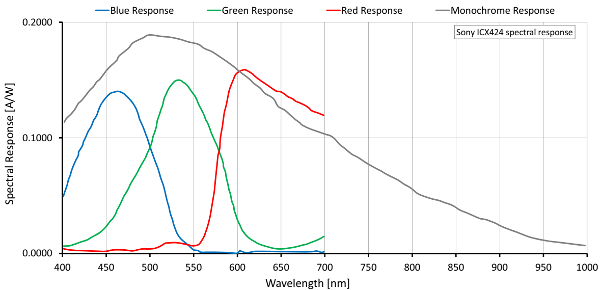
Figure 7: Mako G-032 (Sony ICX424) spectral response
