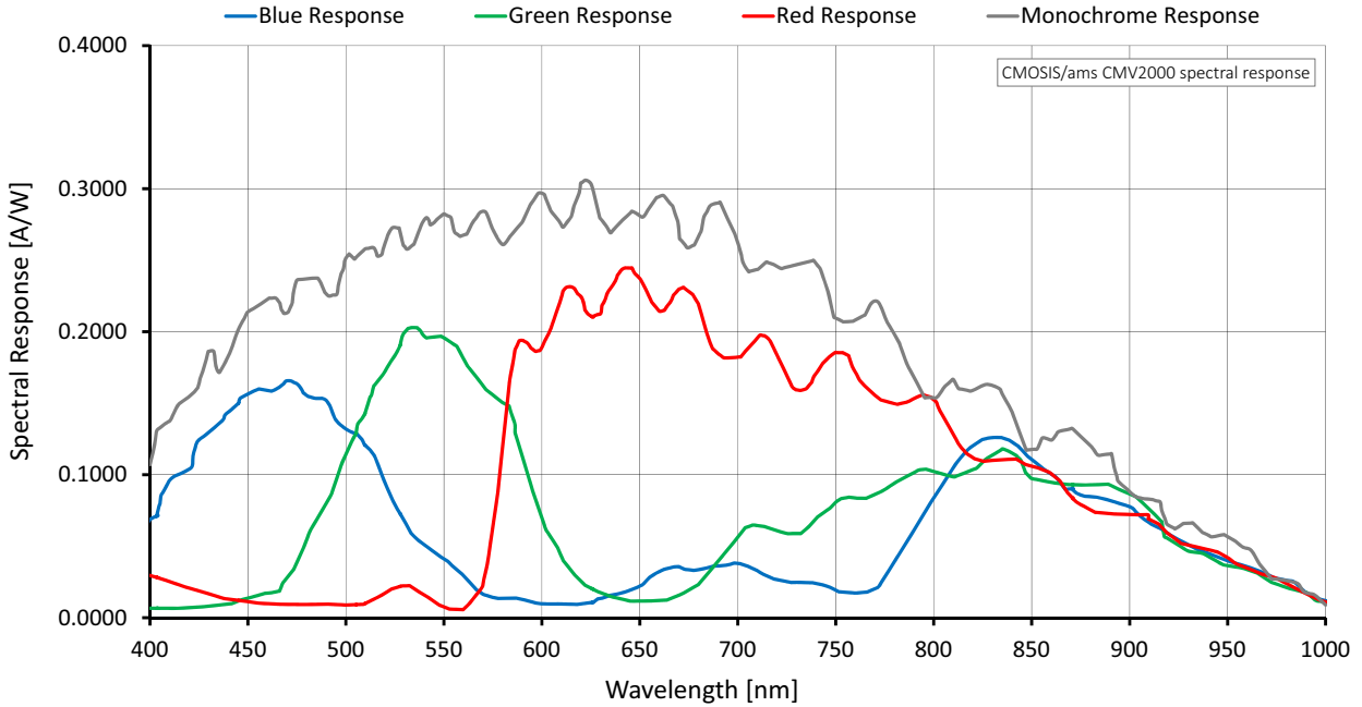
Figure 26: Mako G-223 (CMOSIS/ams CMV2000) spectral response
