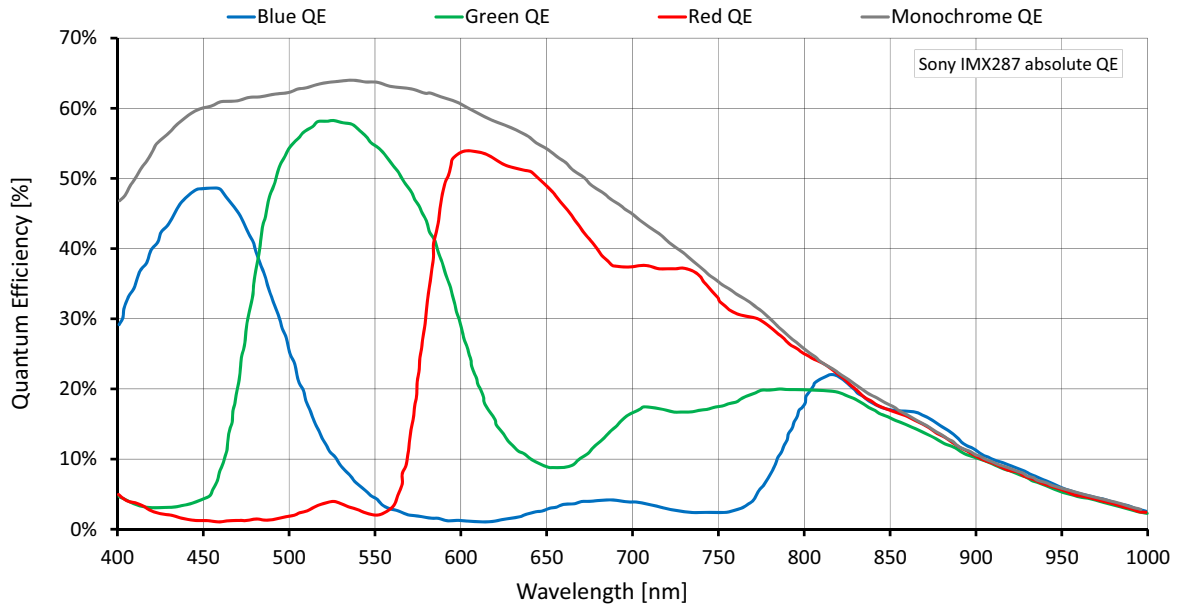
Figure 9: Mako G-040 (Sony IMX287) absolute QE
