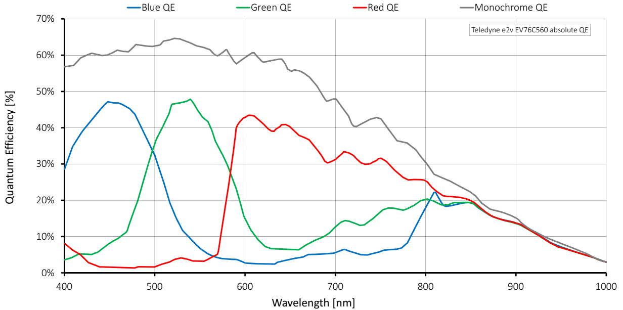
Figure 15: Mako G-131 (Teledyne e2v EV76C560) absolute QE
