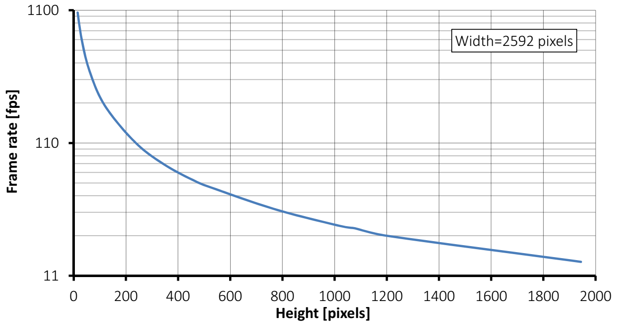
Figure 43: Mako G-503 frame rate as a function of ROI height
