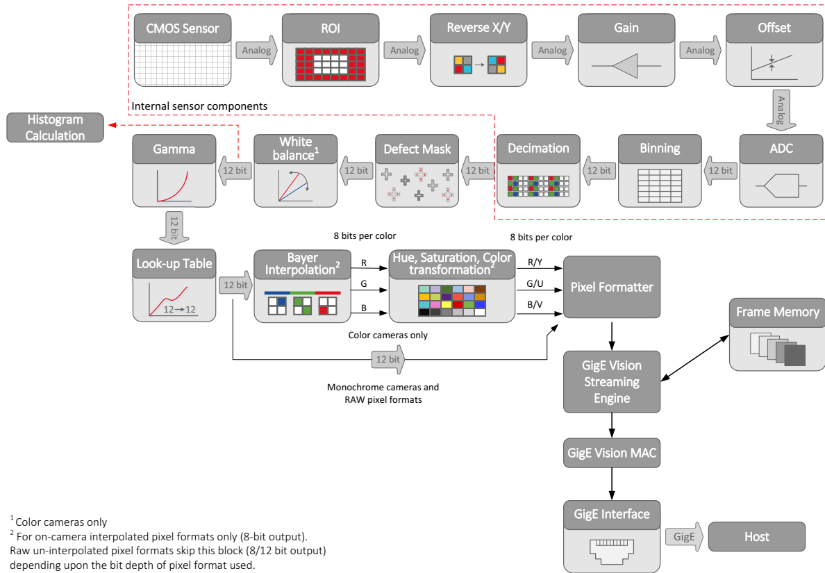
Figure 77: Mako G-503 series image data flow
