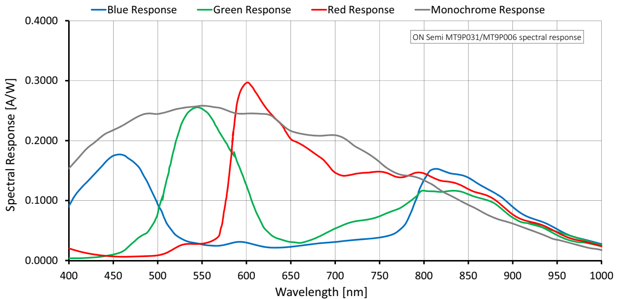
Figure 42: Mako G-503 (ON Semi MT9P031/MT9P006) spectral response
