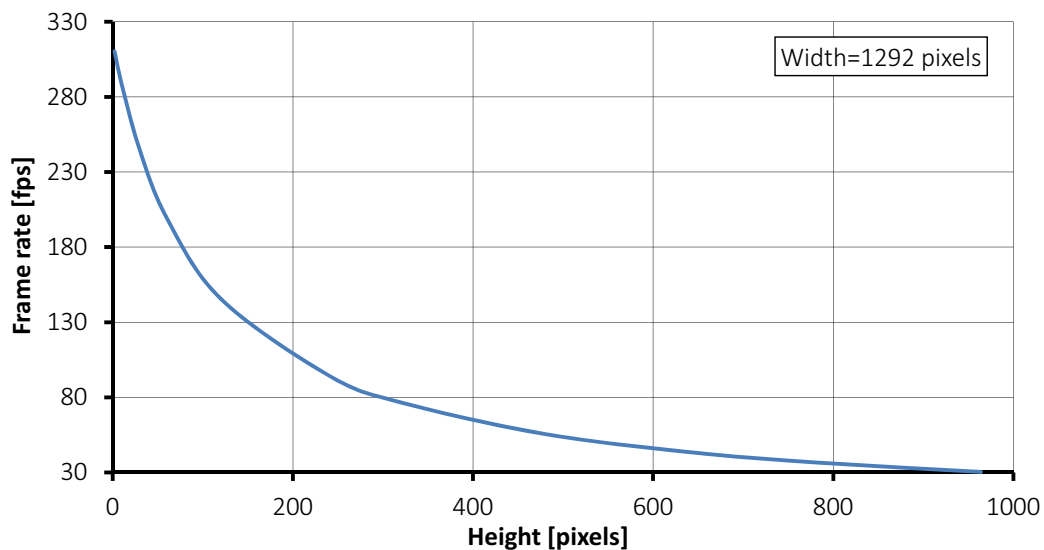
Figure 14: Mako G-125 frame rate as a function of ROI height
