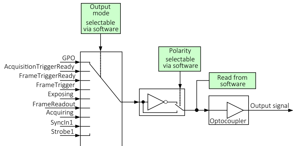
Figure 69: Output block diagram
