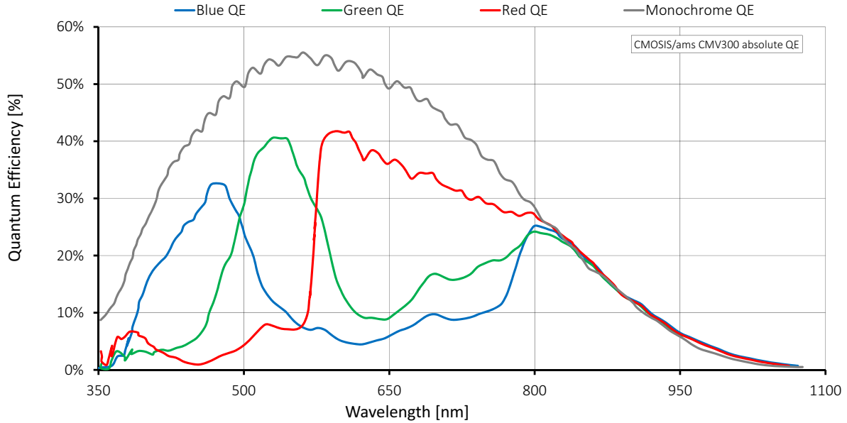
Figure 3: Mako G-030 (CMOSIS/ams CMV300) absolute QE
