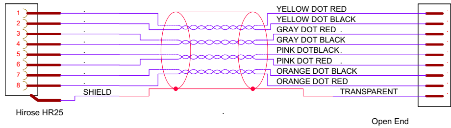
Figure 63: Mako G cable color coding
