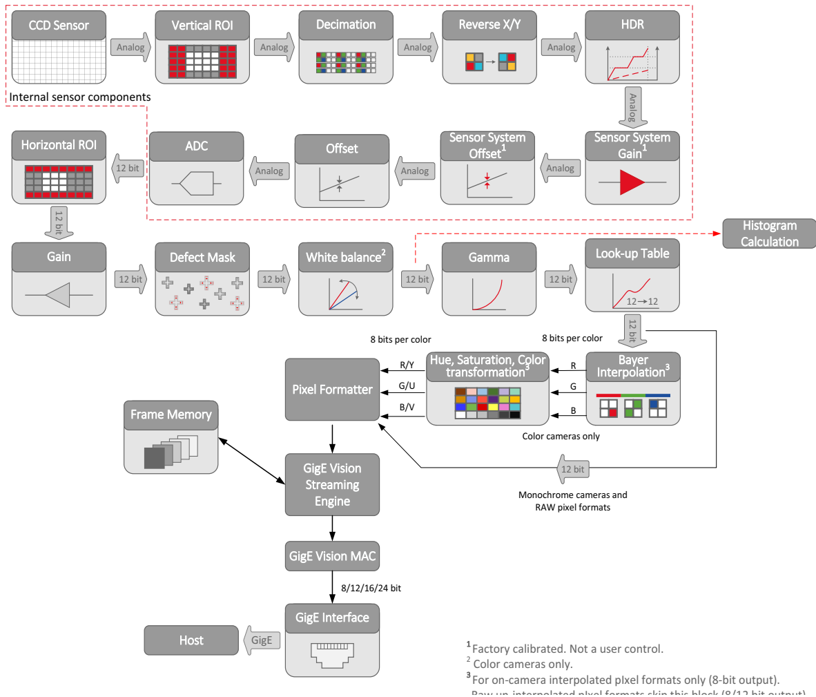
Figure 73: Mako G-030 series image data flow
