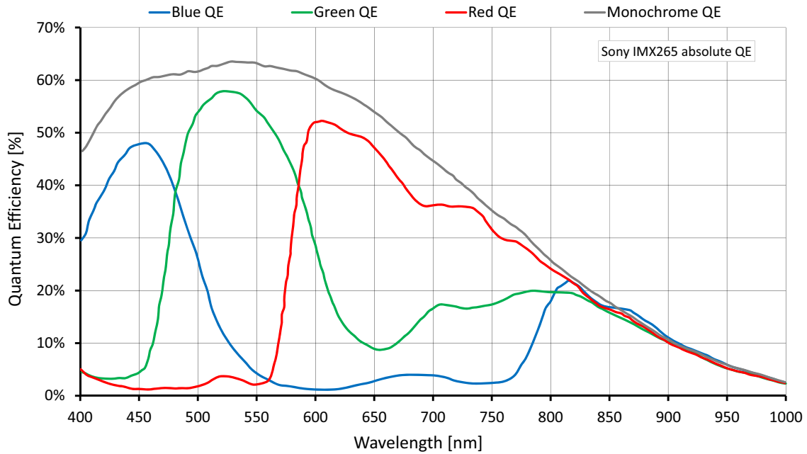
Figure 33: Mako G-319 (Sony IMX265) absolute QE
