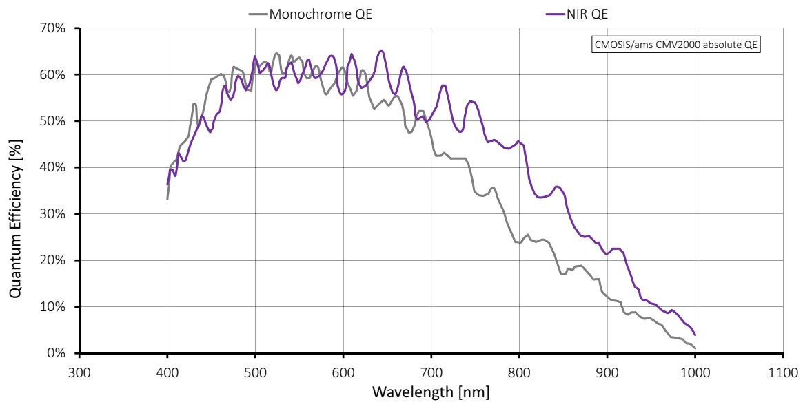
Figure 25: Mako G-223B NIR (CMOSIS/ams CMV2000) absolute QE
