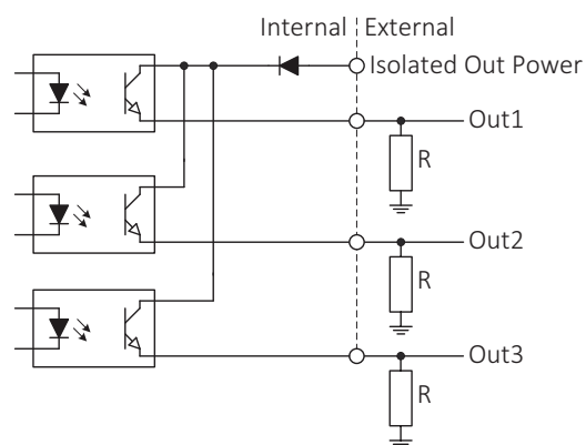
Figure 66: Output block diagram
