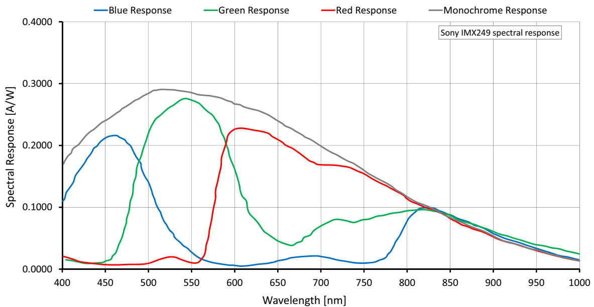
Figure 30: Mako G-234 (Sony IMX249) spectral response
