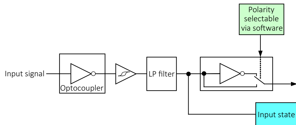
Figure 68: Input block diagram
