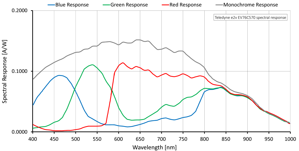
Figure 22: Mako G-192 (Teledyne e2v EV76C570) absolute QE
