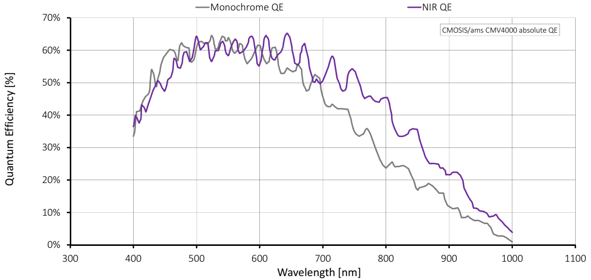
Figure 37: Mako G-419B NIR (CMOSIS/ams CMV4000) absolute QE
