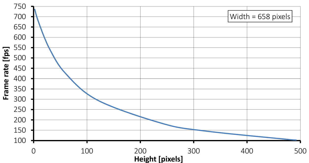
Figure 8: Mako G-032 frame rate as a function of ROI height
