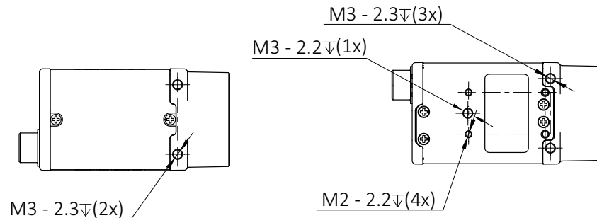
Figure 2: Mounting threads on top and bottom of housing
