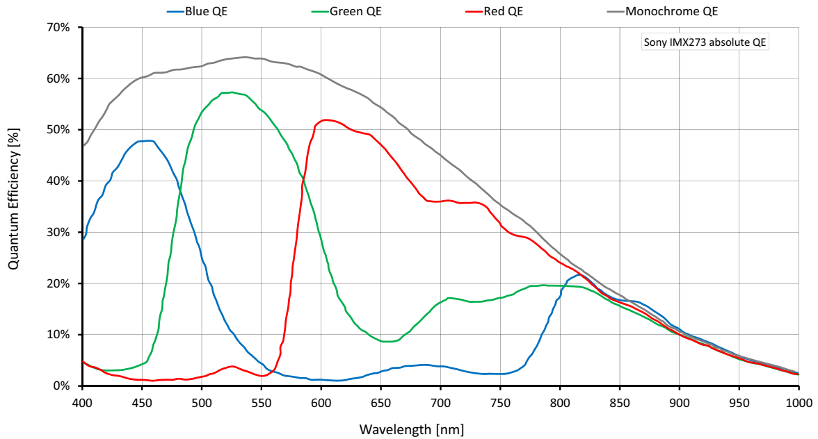
Figure 18: Mako G-158 (Sony IMX273) absolute QE
