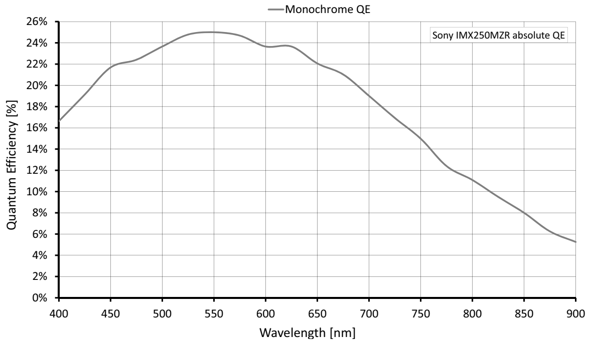
Figure 47: Mako G-508B POL (Sony IMX250MZR) absolute QE
