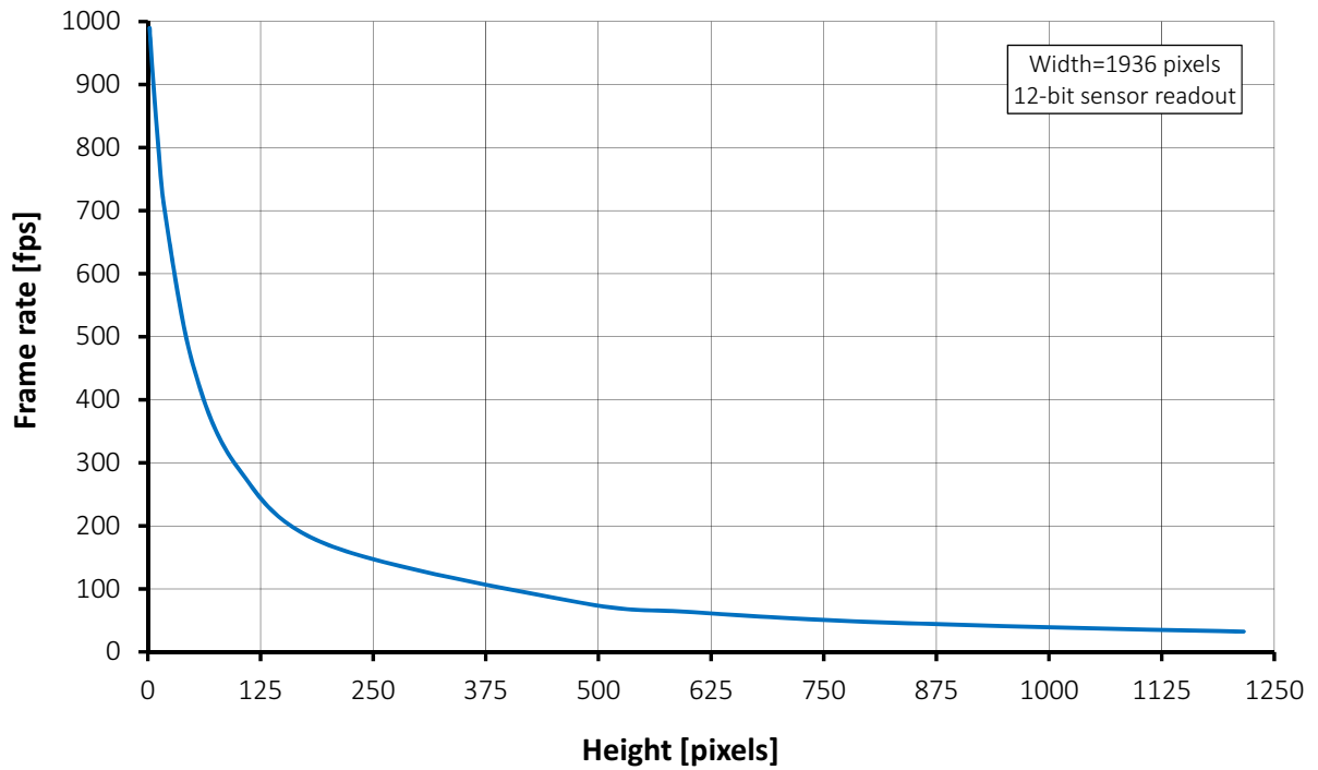
Figure 31: Mako G-234 12-bit sensor frame rate as a function of ROI height
