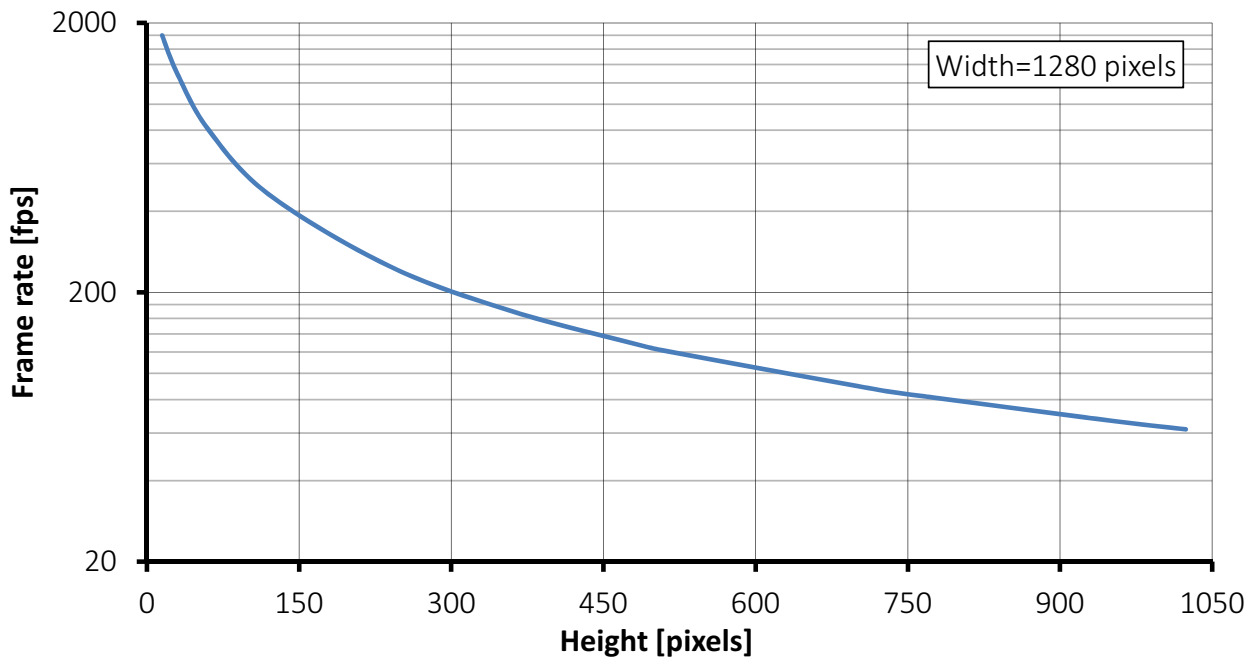
Figure 17: Mako G-131 frame rate as a function of ROI height
