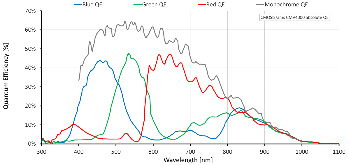
Figure 36: Mako G-419 (CMOSIS/ams CMV4000) absolute QE
