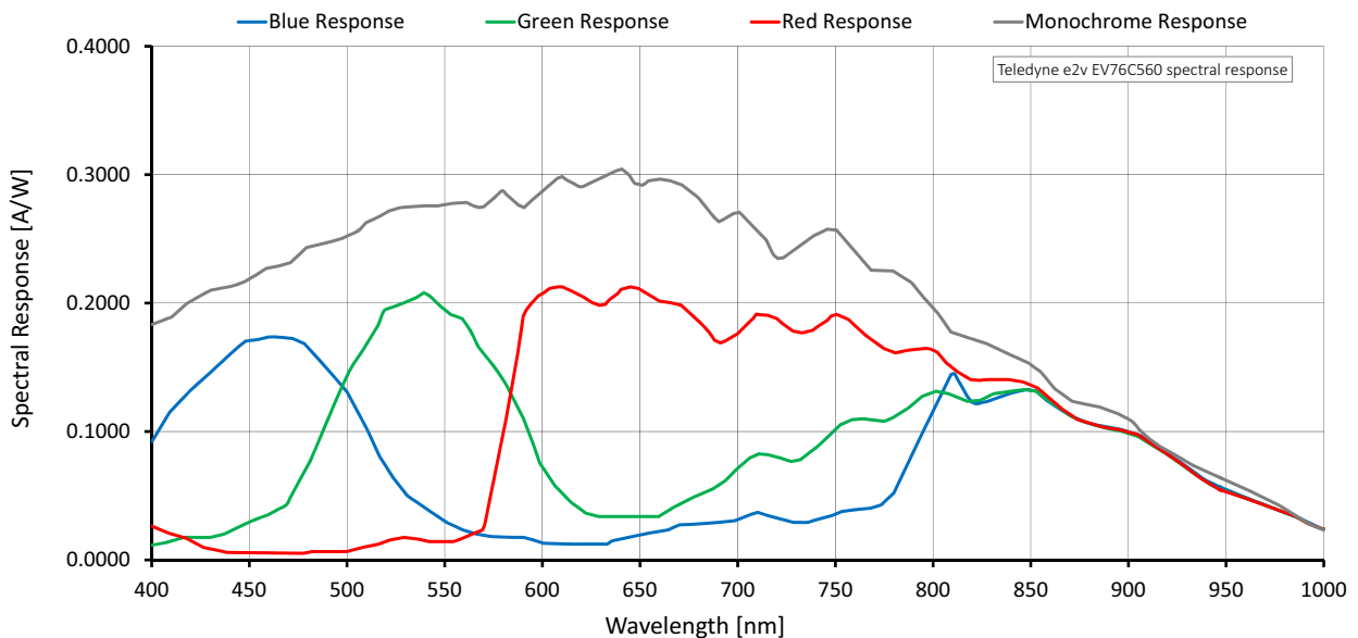
Figure 16: Mako G-131 (Teledyne e2v EV76C560) spectral response
