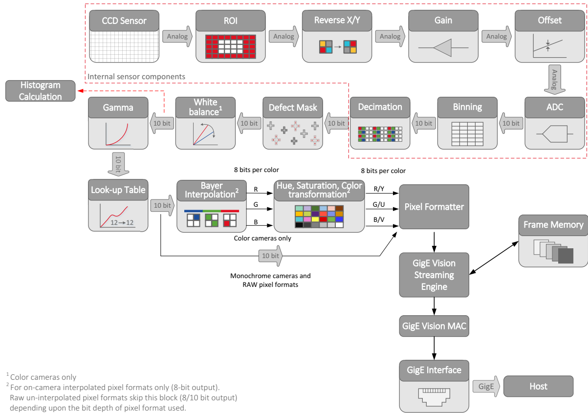
Figure 74: Mako G-131 and G-192 series image data flow
