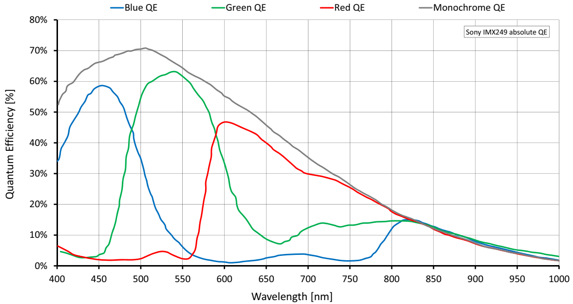
Figure 29: Mako G-234 (Sony IMX249) absolute QE
