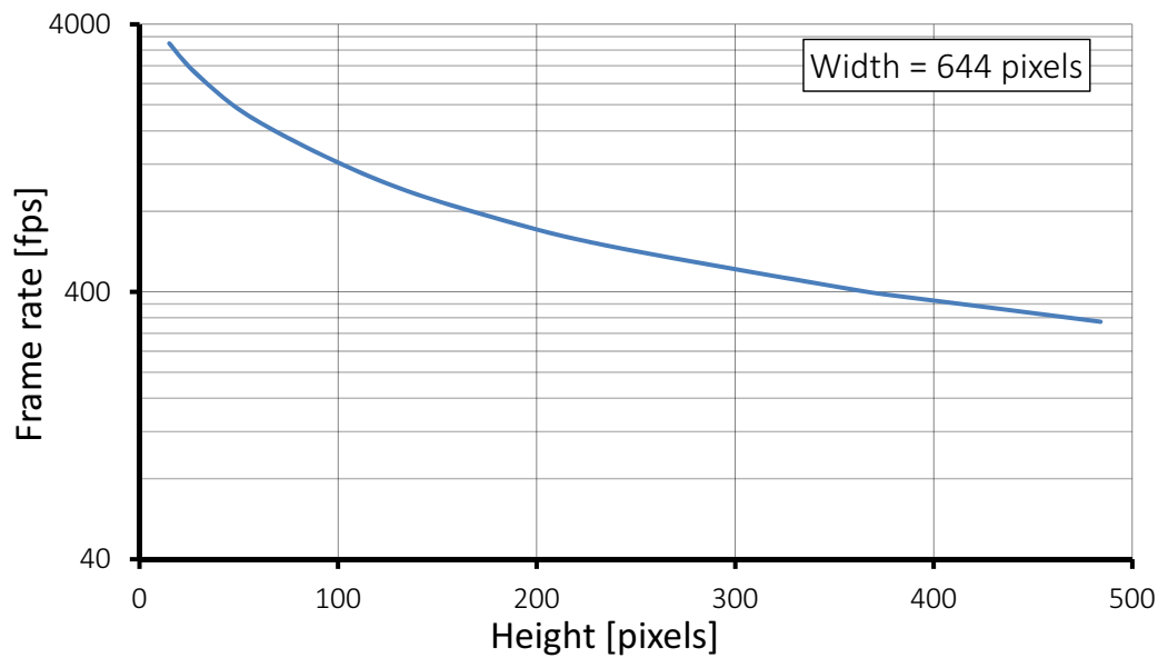
Figure 5: Mako G-030 frame rate as a function of ROI height
